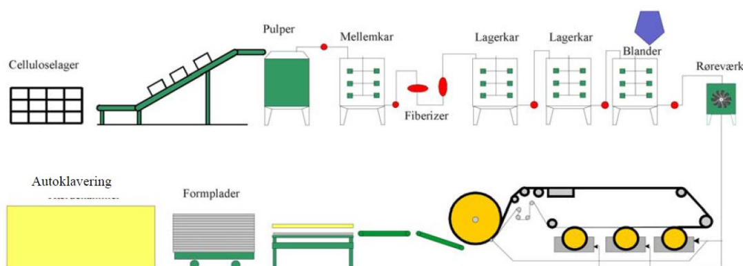
Fig. 3 : Diagram of fibre cement production (here Hatschek and autoclaving) 13
